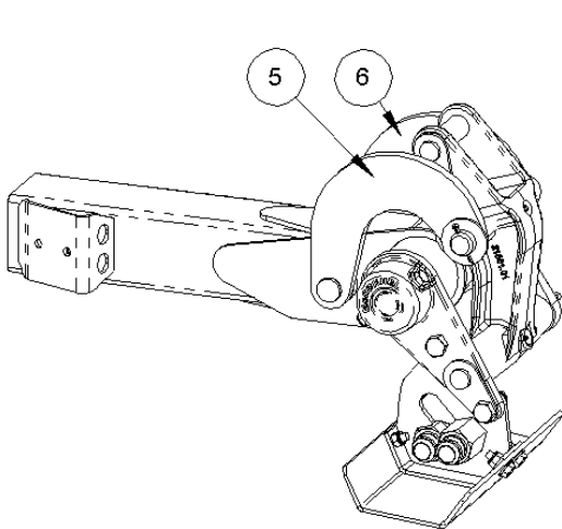
SHOWN ASEMBLED FOR LH
