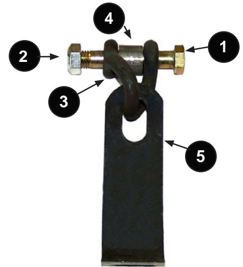
LBG Assembly
