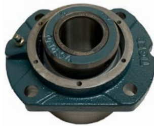
FLANGE BEARING GROUND ROLLER SUPER DUTY SIDE AND REAR FLAIL - 1 3/8" Part # 06520028
