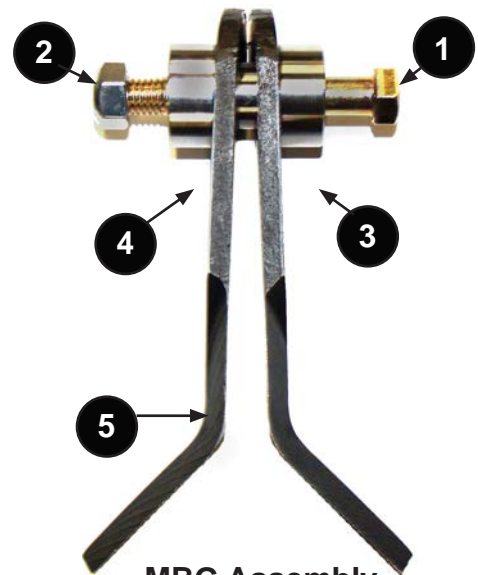
MBG Assembly
