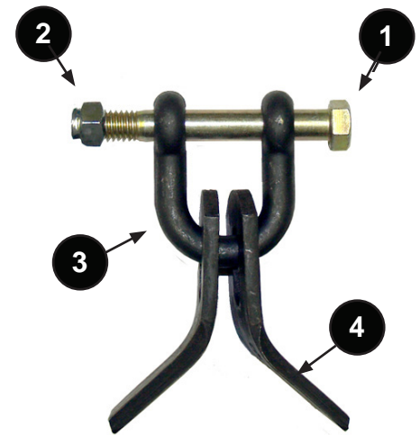
Grass Only Assembly
