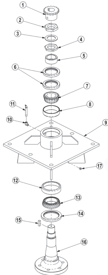
COMPLETE SPINDLE - PART# 6T1024H5
