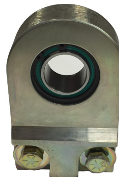
CLEVIS WITH SPHERICAL BEARING- ATTACHES TO 3 1/2" X 20" CYLINDER Part # TB3033
